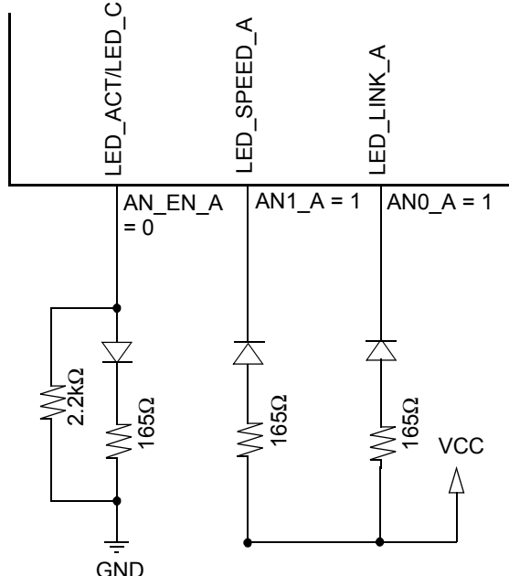
Figure 3. AN Strapping and LED Loading Example
