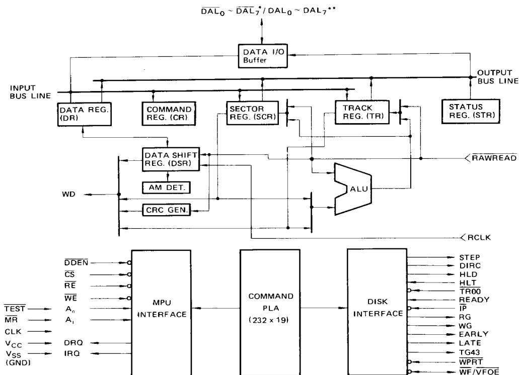
MB8876A/MB8877A BLOCK DIAGRAM
