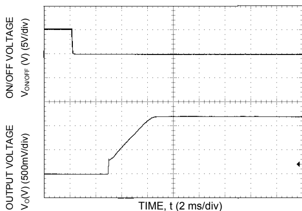
Figure 11. Typical Start-up Using On/Off Voltage ( I_o = I_{o,max} , V_{IN} = 8V ).
