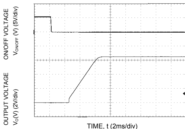
Figure 41. Typical Start-up Using On/Off Voltage ( I_o = I_{o,max} ).
