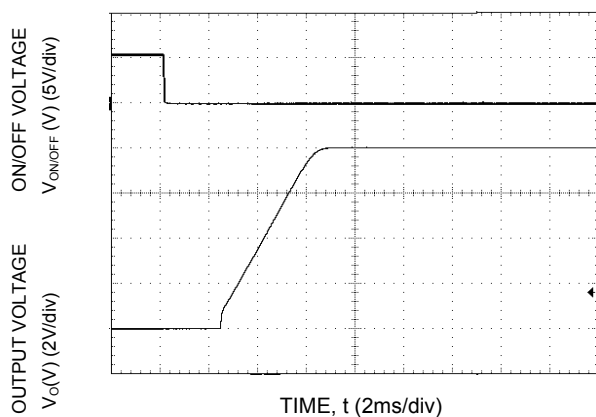
Figure 47. Typical Start-up Using On/Off Voltage ( I_o = I_{o,max} ).
