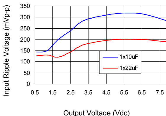
Figure 52. Input ripple voltage for various output voltages with 1 \times 10 \mu F or 1 \times 22 \mu F ceramic capacitors at the input (4A load). Input voltage is 12V.
