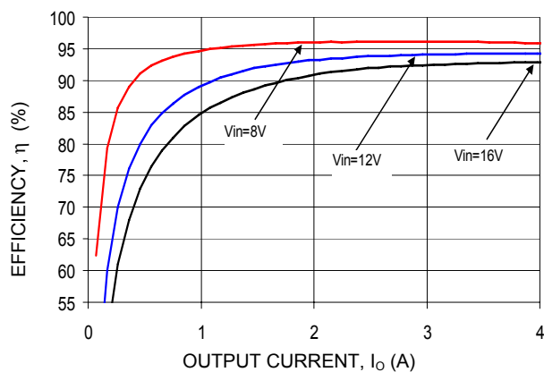
Figure 37. Converter Efficiency versus Output Current.
