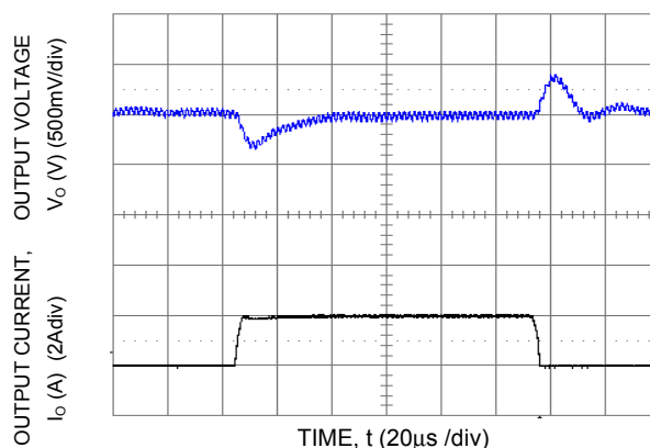
Figure 34. Transient Response to Dynamic Load Change from 0% 50% to 0%.
