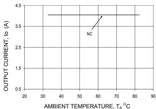
Figure 31. Derating Output Current versus Ambient Temperature and Airflow.
