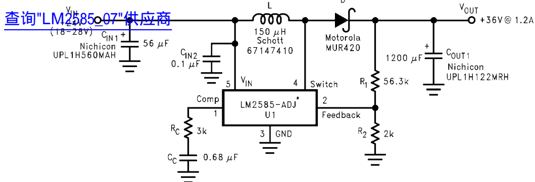
FIGURE 36. +24V to +36V Boost Regulator
