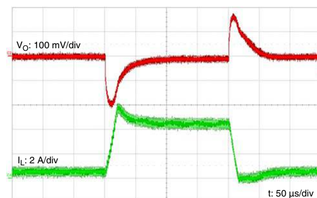
Transient response. V_{IN} = 12\text{ V} , V_O = 3.3\text{ V} and L = 10\text{ μH} (IHLP2525EZ type). C_O consists of MLCC of 4.7 \mu\text{F} and tantalum of 100 \mu\text{F}/20\text{ V} \times 2 . Output current steps up and down between 0.4 A and 4 A with less than 1 \mu\text{s} rising and falling time.
