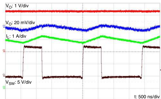
V_O ripple and V_{SW} switching waveform. V_{IN} = 12\text{ V} , V_O = 3.3\text{ V} and L = 10\text{ μH} (IHLP2525EZ type). C_O consists of MLCC of 4.7 \mu\text{F} and tantalum of 100 \mu\text{F}/20\text{ V} \times 2
