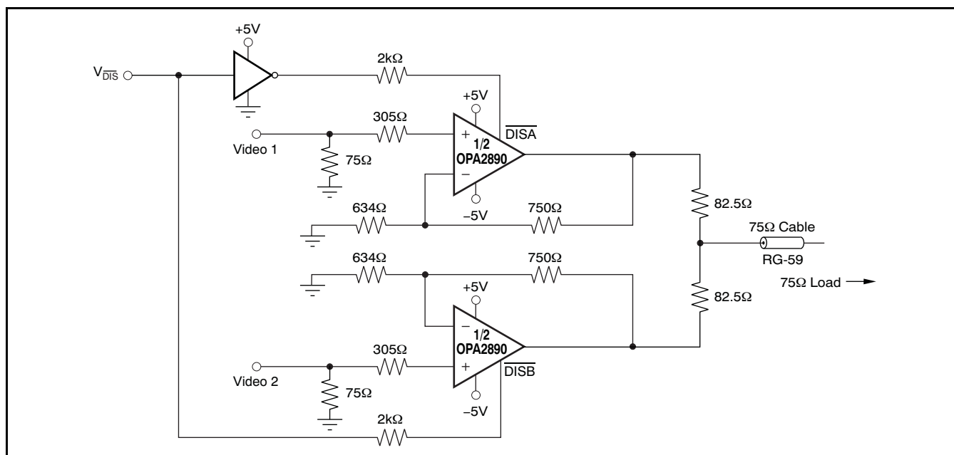
Figure 54. 2-Channel Video Multiplexer (MSOP-10 package only)
