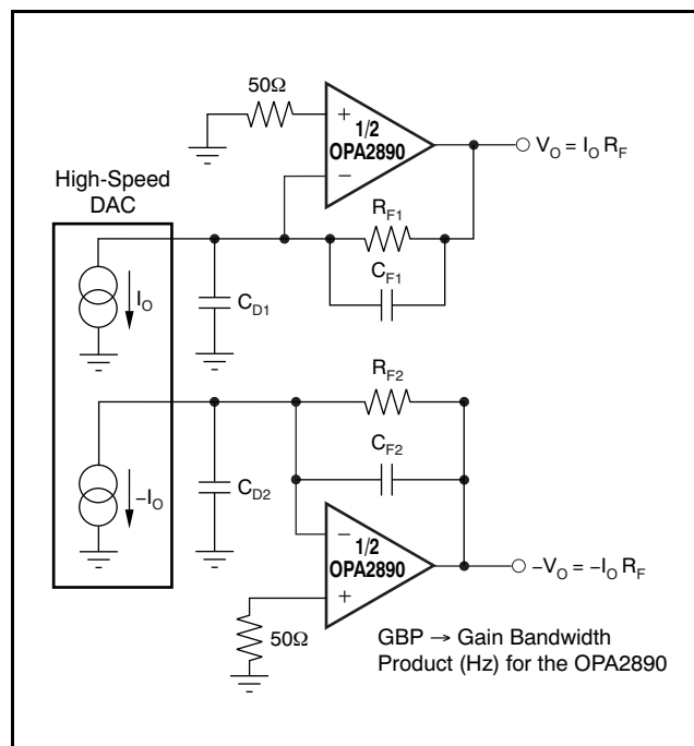
Figure 53. DAC Transimpedance Amplifier
