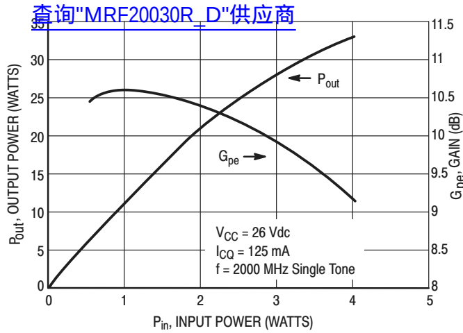
Figure 2. Output Power & Power Gain versus Input Power
