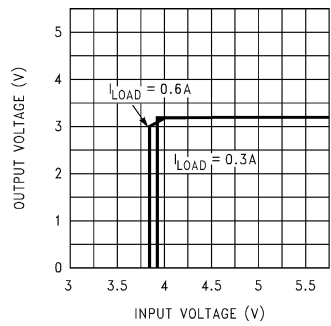
Dropout Voltage—3.3V Option
