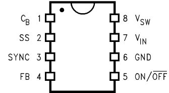
8-Lead Package
