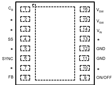
16-Lead LLP Surface Mount Package
