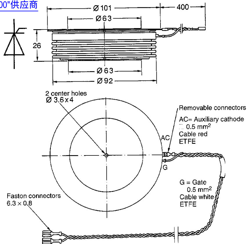
Fig. 12 Device Outline Drawing.
