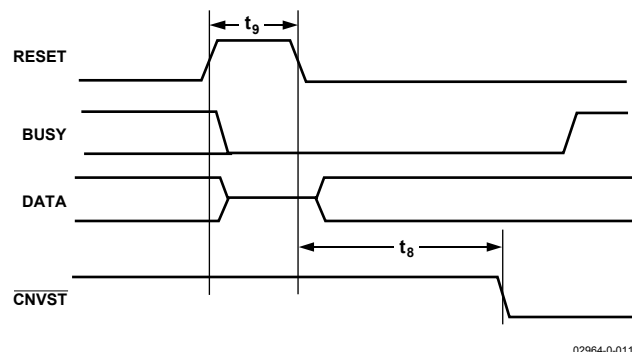
Figure 27. RESET Timing
