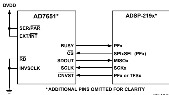
Figure 37. Interfacing the AD7651 to an SPI Interface
