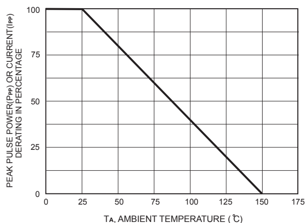
FIG.2-PULSE DERATING CURVE
