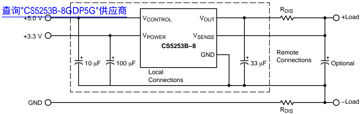
Figure 16. Remote Sense
