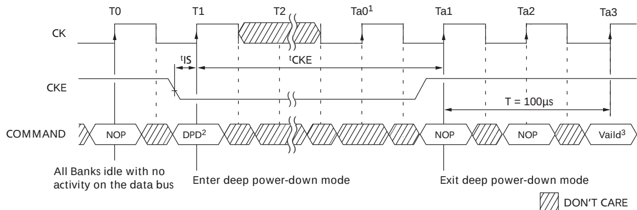
Figure 28: Deep Power-Down
