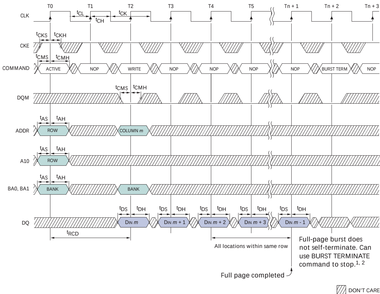
Figure 53: WRITE – Continuous-Page Burst
