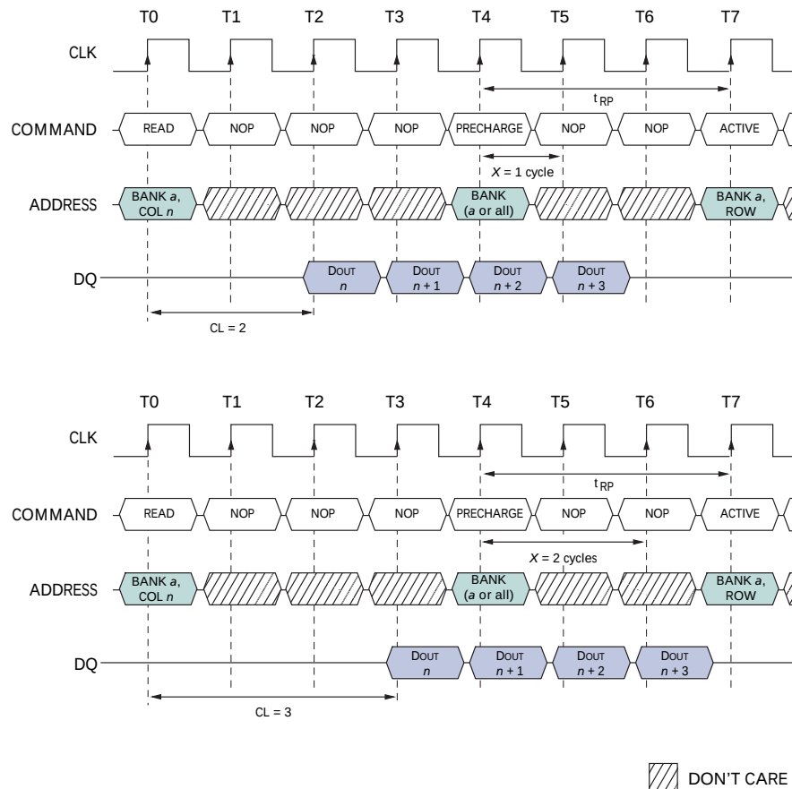
Figure 16: READ-to-PRECHARGE
