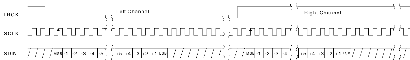
Figure 2. I²S Data
