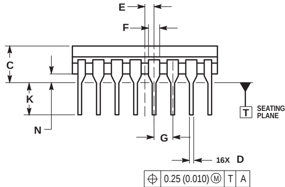
CDIP-16 L SUFFIX CERAMIC DIP PACKAGE CASE 620A-01 ISSUE O
