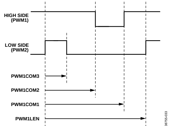
Figure 32. PWM Timing
