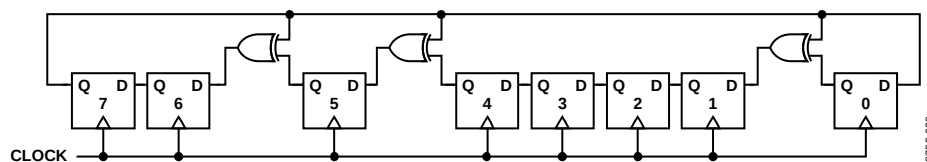
Figure 38. 8-Bit LFSR
