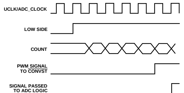
Figure 33. ADC Conversion
