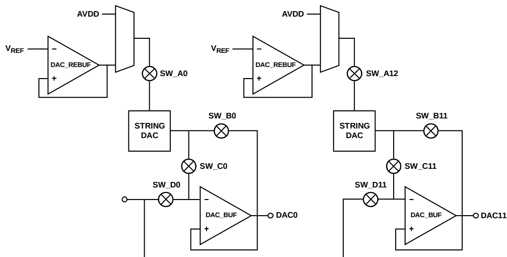
Figure 27. DAC Configuration
