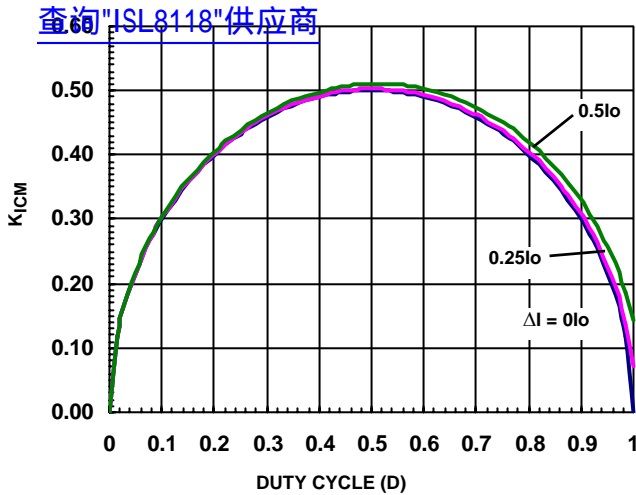
FIGURE 12. INPUT-CAPACITOR CURRENT MULTIPLIER FOR SINGLE-PHASE BUCK CONVERTER
