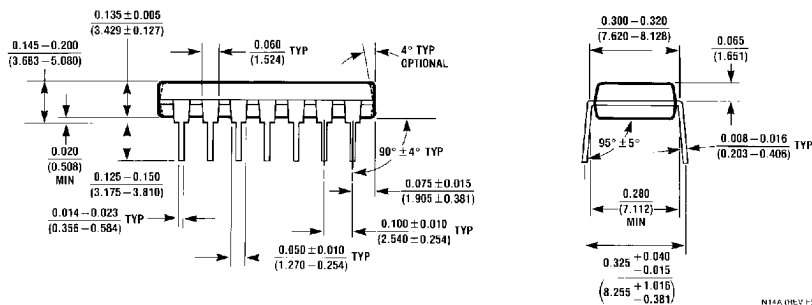
14 Lead Plastic Dual-In-Line Package (P) NS Package Number N14A
