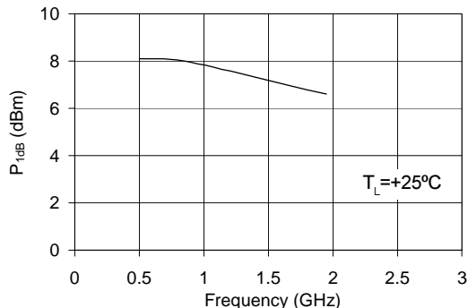
P 1dB vs. Frequency V D = 2.6 V, I D = 20 mA
