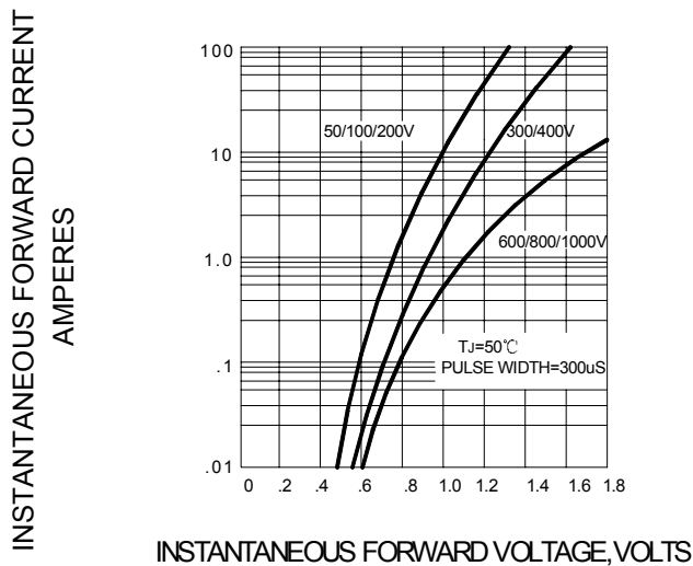
FIG.3-TYPECAL FORWARD CHARACTERISTICS
