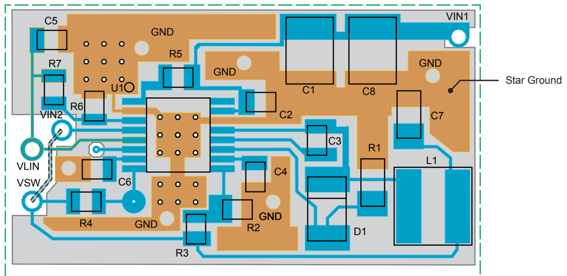
PCB Layout Diagram
