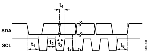
Figure 24. I 2 C Timing Diagram
