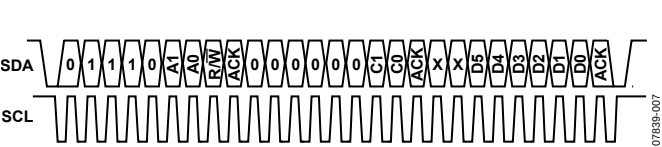
Figure 23. I 2 C 3-Byte Timing Sequence
