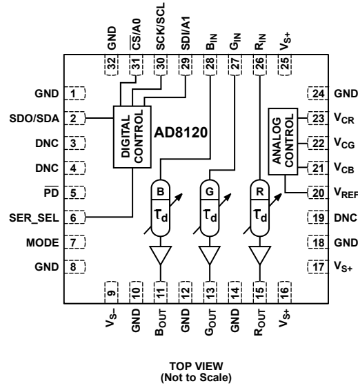
Figure 3. Pin Configuration
