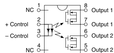
LCA210L Pinout
