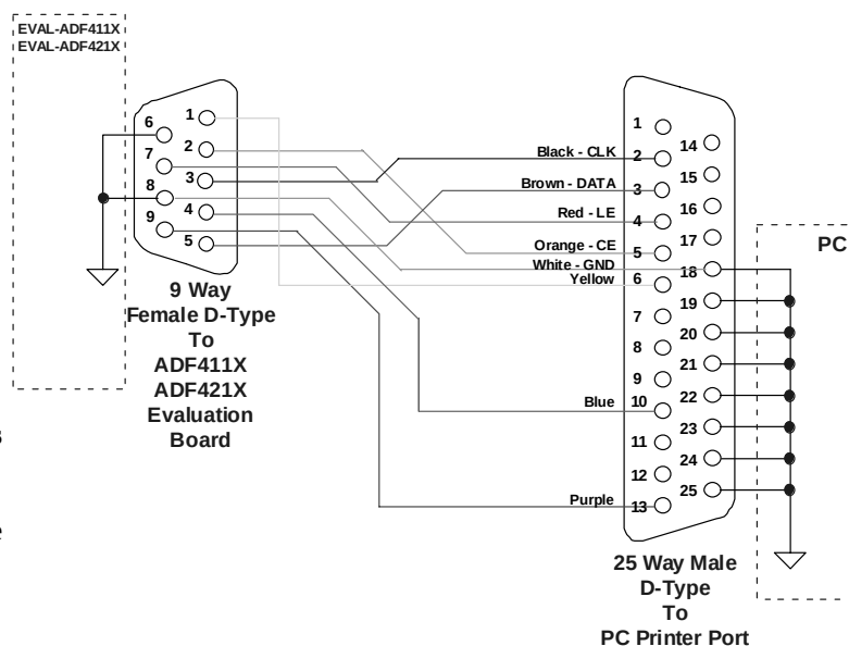
ADF411X/ADF421X CABLE CONNECTIONS Rev 2 (15/3/99)
