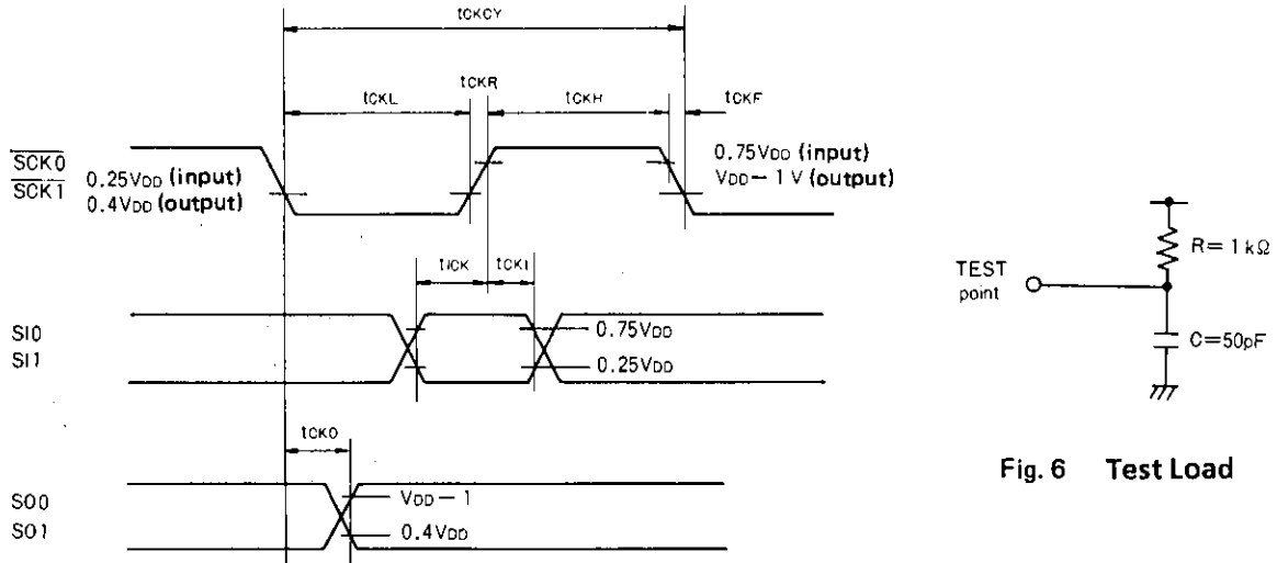
Fig. 5 Serial Input/Output Timing
