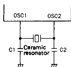
Fig. 2 Ceramic Resonator OSC Circuit
