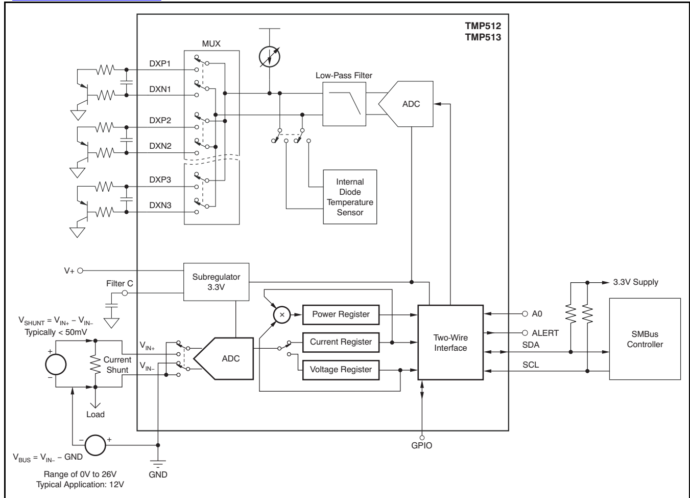
Figure 27. TMP512/13 Configured for Shunt and Bus Voltage Measurement
