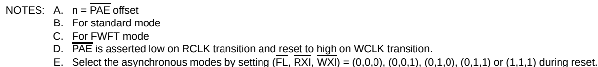
Figure 9. Asynchronous Programmable Almost-Empty-Flag Timing (Standard and FWFT Modes)
