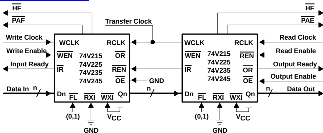
Figure 27. Block Diagram of 1024 \times 18 , 2048 \times 18 , 4096 \times 18 , 8192 \times 18 Synchronous FIFO Memory With Programmable Flags Used in Depth-Expansion Configuration
