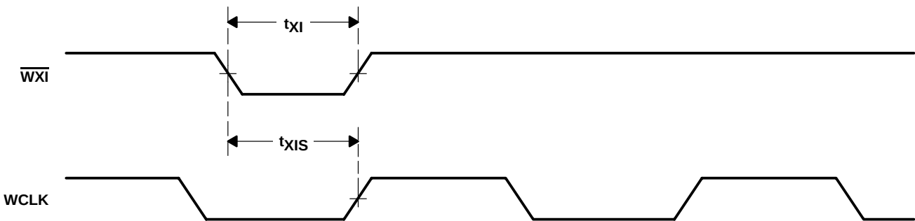
Figure 14. Write-Expansion-In Timing
