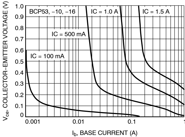
Figure 9. BCP53, -10, -16 Saturation Region
