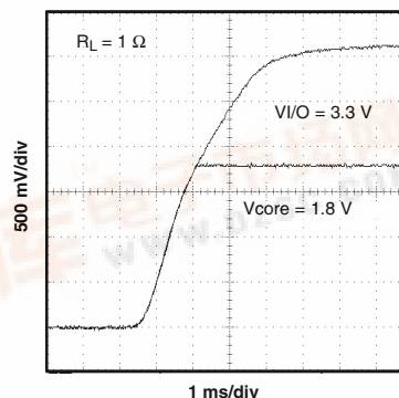
START-UP WAVEFORM
