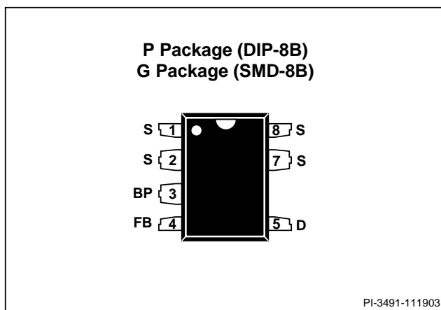
Figure 3. Pin Configuration.
