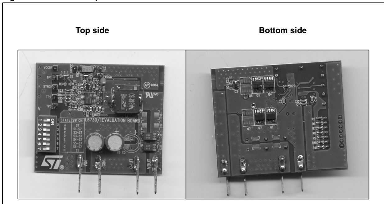
Figure 29. Demoboard picture.
