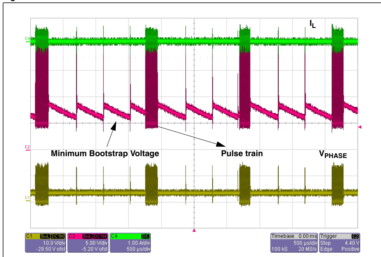
Figure 24. 12V \rightarrow 3.3V@0A in no-sink
