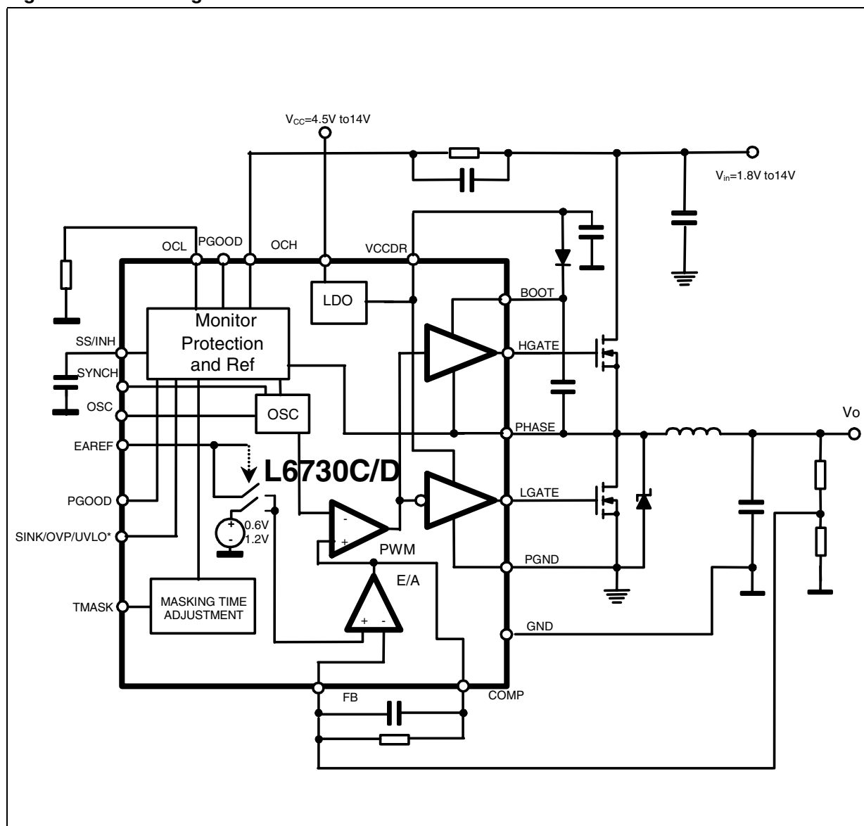
Figure 1. Block diagram
