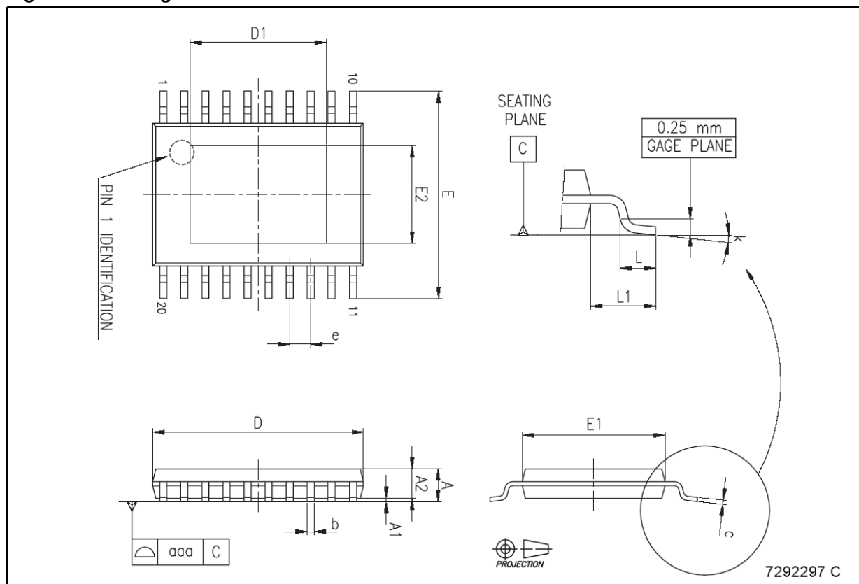
Figure 42. Package dimensions
