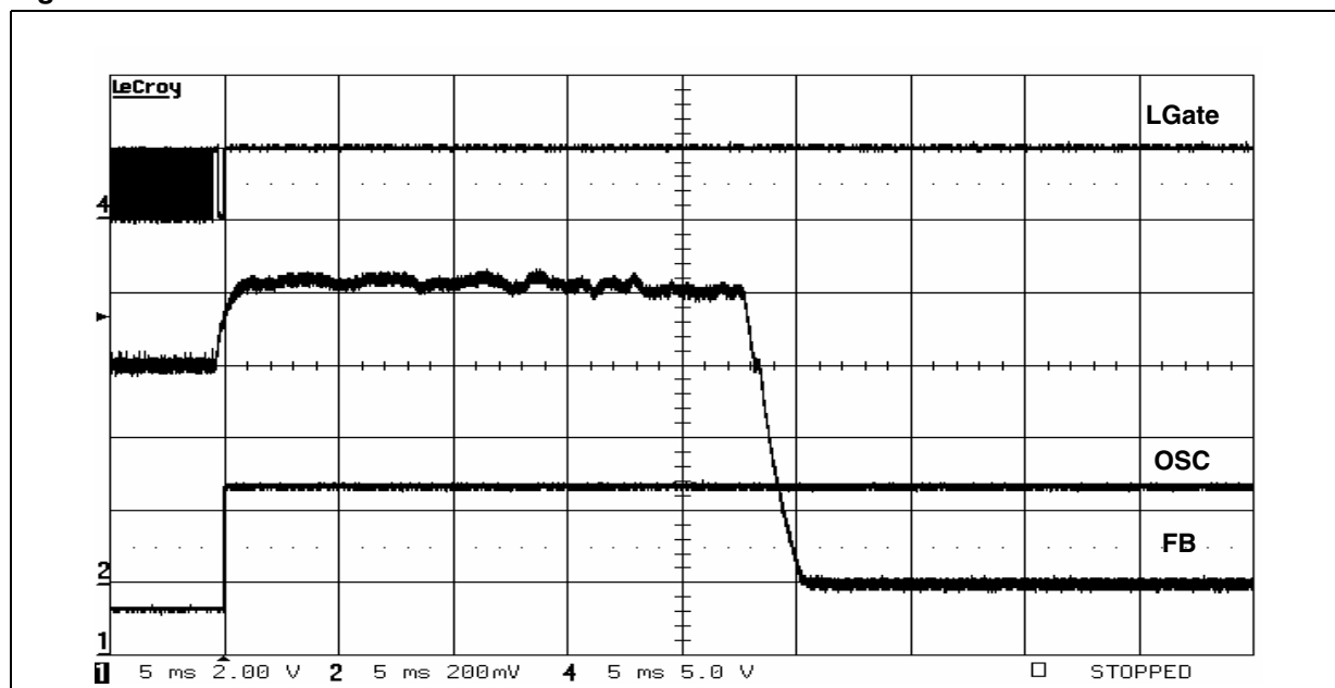
Figure 13. OVP latched
