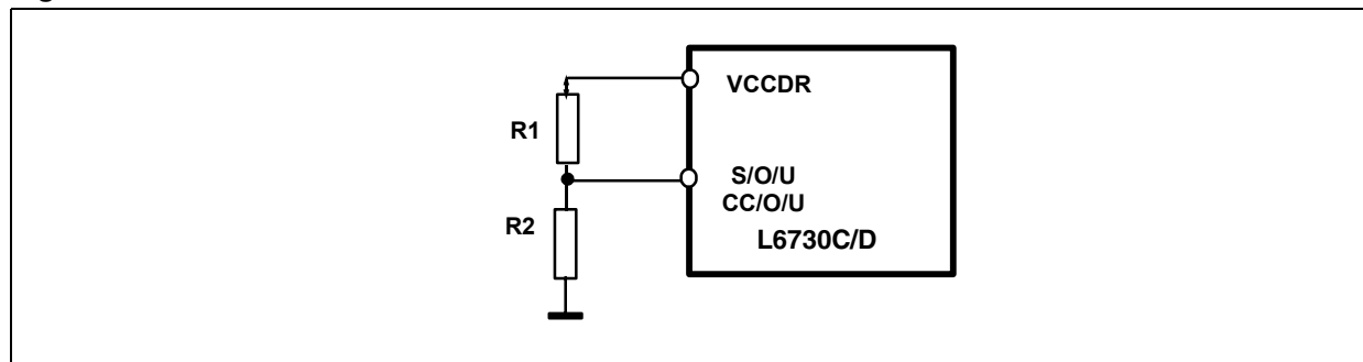
Figure 20. External resistor
