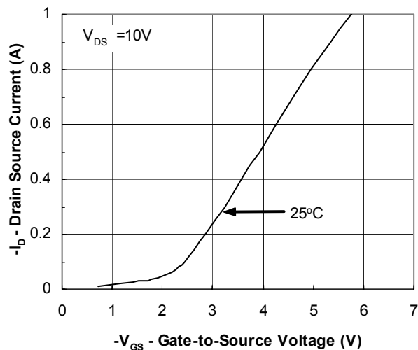
Fig. 2. Transfer Characteristics
