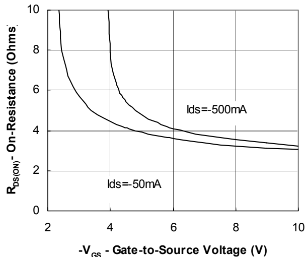
Fig. 4. On-Resistance vs. G-S Voltage
