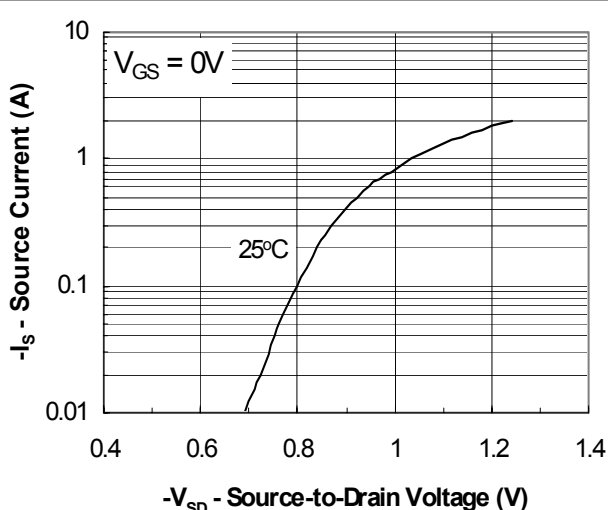
Fig. 6. Source-Drain Diode Forward Voltage
