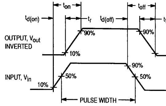
Figure 18. Inductive Switching Time Test Circuit and Timing Chart
