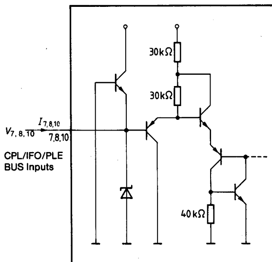
Test circuit 2
