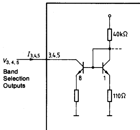
Test circuit 3
