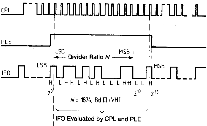
Pulse diagram
