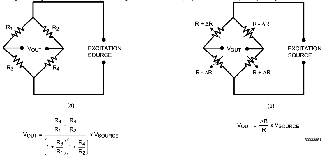
30033850 FIGURE 4. Bridge Sensor
