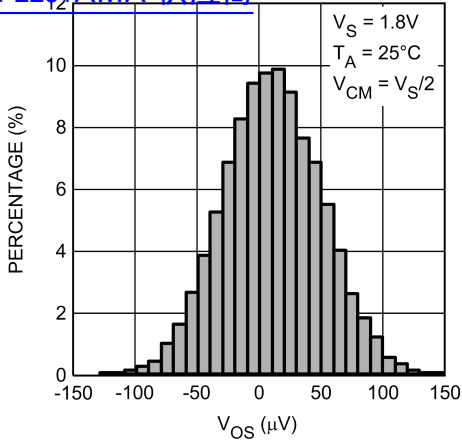
Offset Voltage Distribution 查询"LMP2231"供应商
