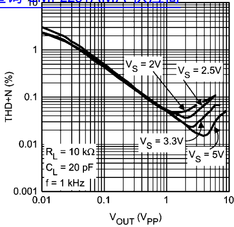
THD+N vs. Amplitude 查询"LMP2231AMA"供应商
