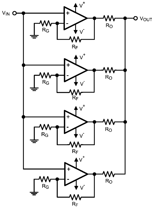
Figure 2 shows a schematic of this input voltage noise reduction circuit. Typical resistor values are: R_G = 10\Omega , R_F = 1\text{ k}\Omega , and R_O = 1\text{ k}\Omega .
