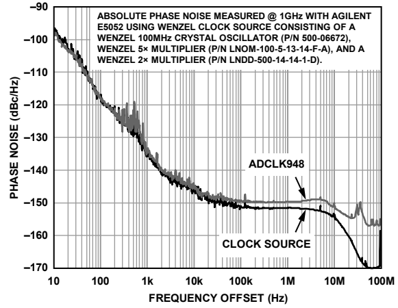
Figure 11. Absolute Phase Noise Measured @ 1 GHz
