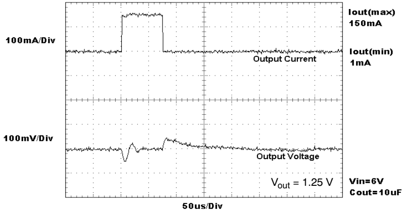
Figure 30. Load Transient Response (10 \mu F)
