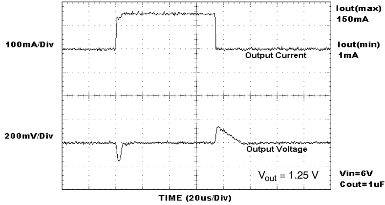
Figure 29. Load Transient Response (1.0 \mu F)
