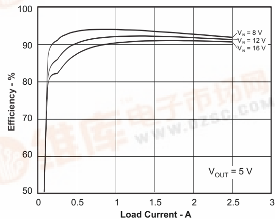
Figure 2. Typical Efficiency of Application Circuit 1 (Described in Application 1)
