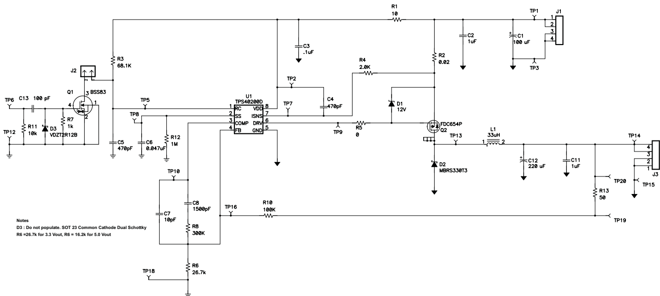
Figure 34. 8-V to 16-V V_{IN} Step-Down Buck Converter
