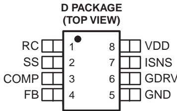
Figure 4. Device Pinout
