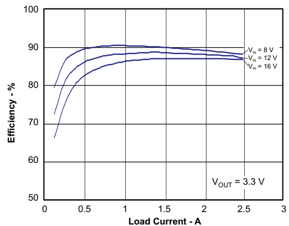
Figure 36. Full-Load Efficiency at 3.3-V V_{OUT}
