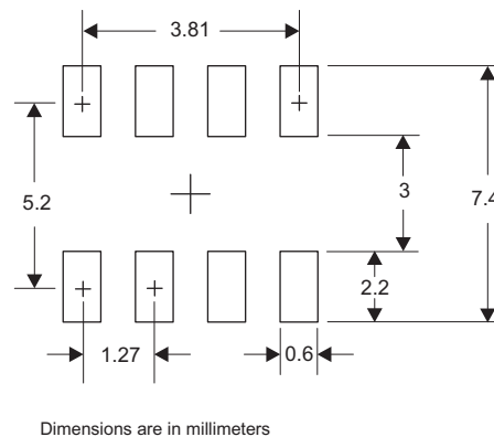
Figure 52. Suggested SOIC-8 PCB Footprint
