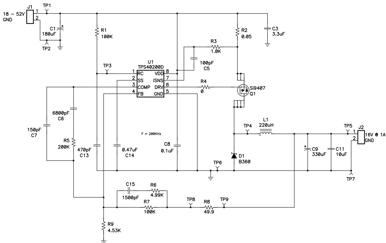
Figure 46. Buck Converter: V_{IN} = 18\text{ V to }50\text{ V} , V_{OUT} = 16\text{ V at }1\text{ A}
