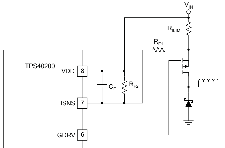
Figure 30. Current-Limit Adjustment
