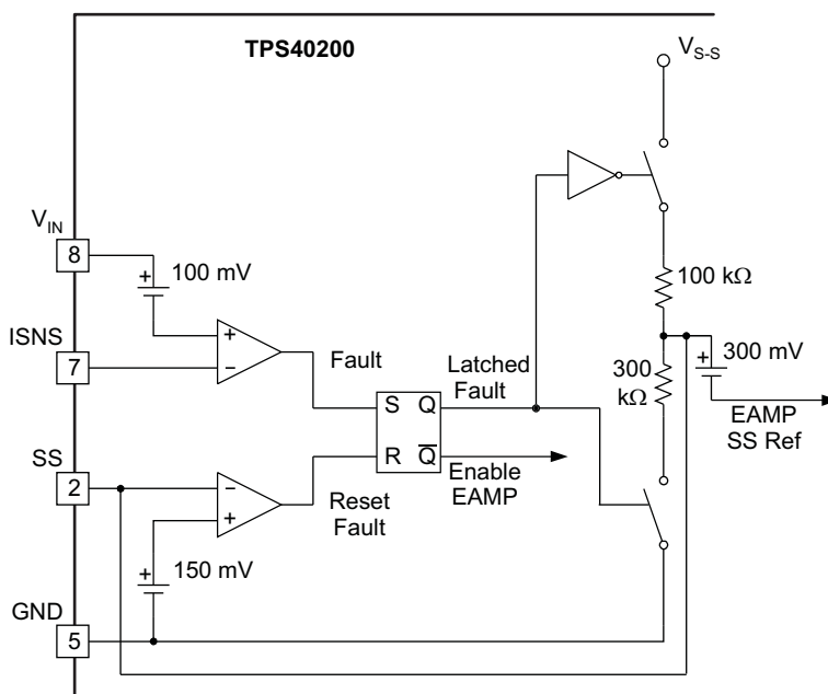
Figure 29. Current-Limit Reset
