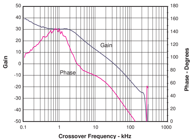
Figure 42. Overall System Gain and Phase Response
