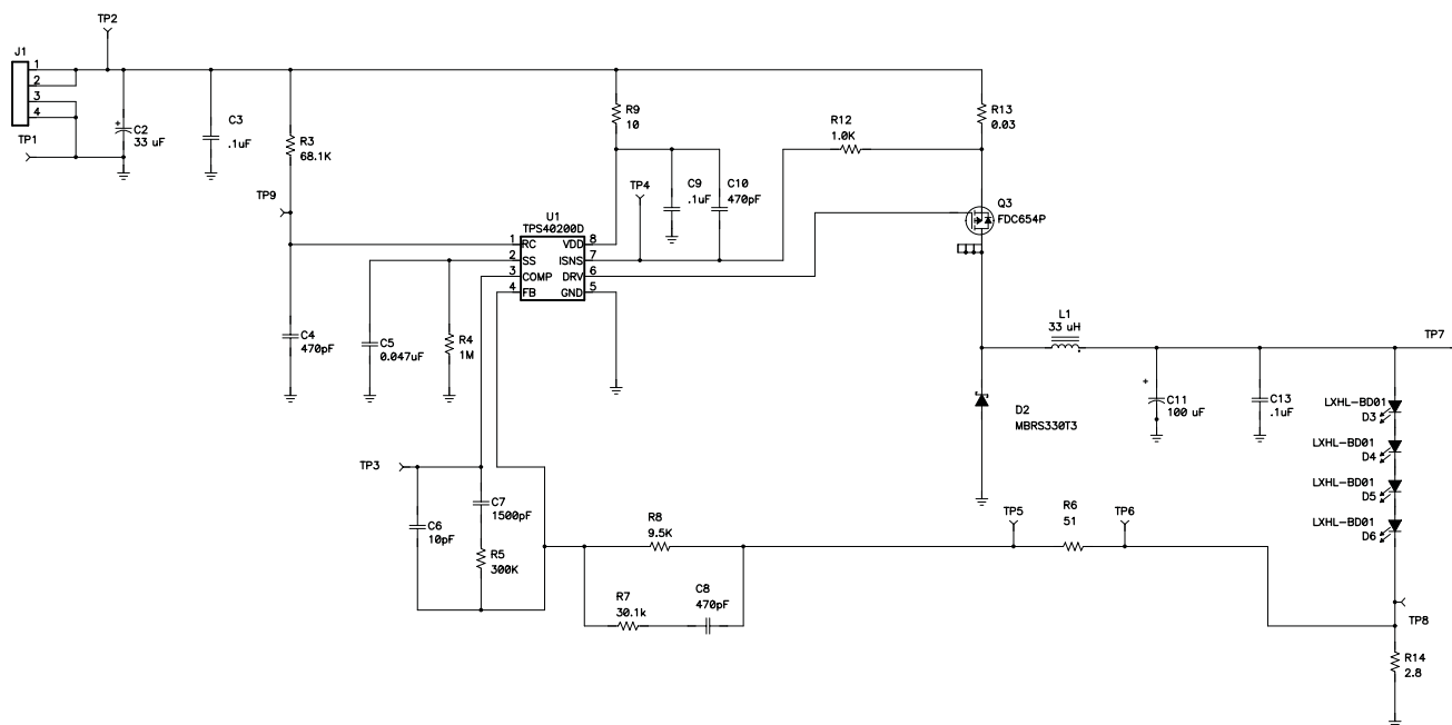
Figure 49. Wide-Input-Voltage Range LED Driver
