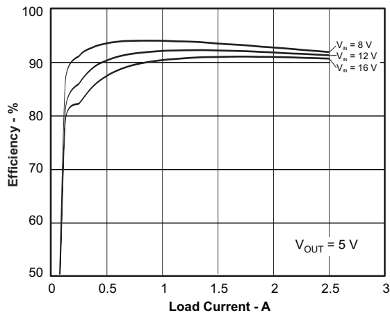
Figure 35. Full-Load Efficiency at 5-V V_{OUT}
