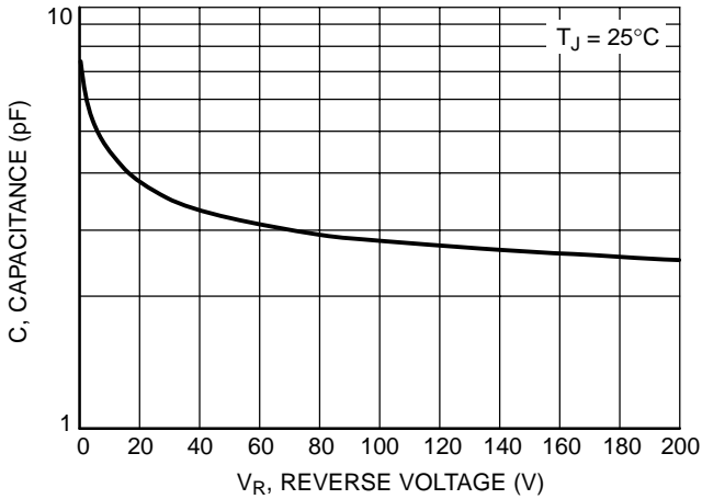
Figure 3. Typical Capacitance
