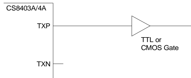
Figure A3. TTL/CMOS Output Circuit
