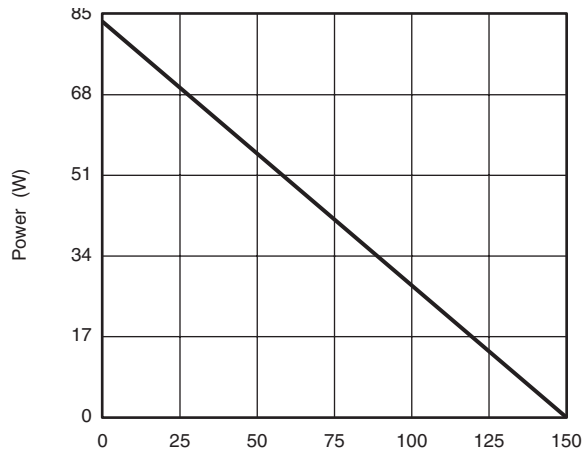
Power, Junction-to-Case
