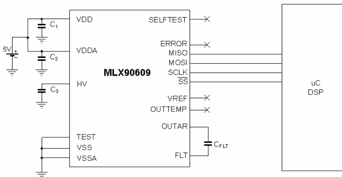
Figure 6-3. MLX90609 with digital output only
