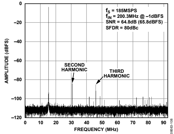
Figure 8. Single-Tone FFT with f_{IN} = 200.3\text{ MHz}
