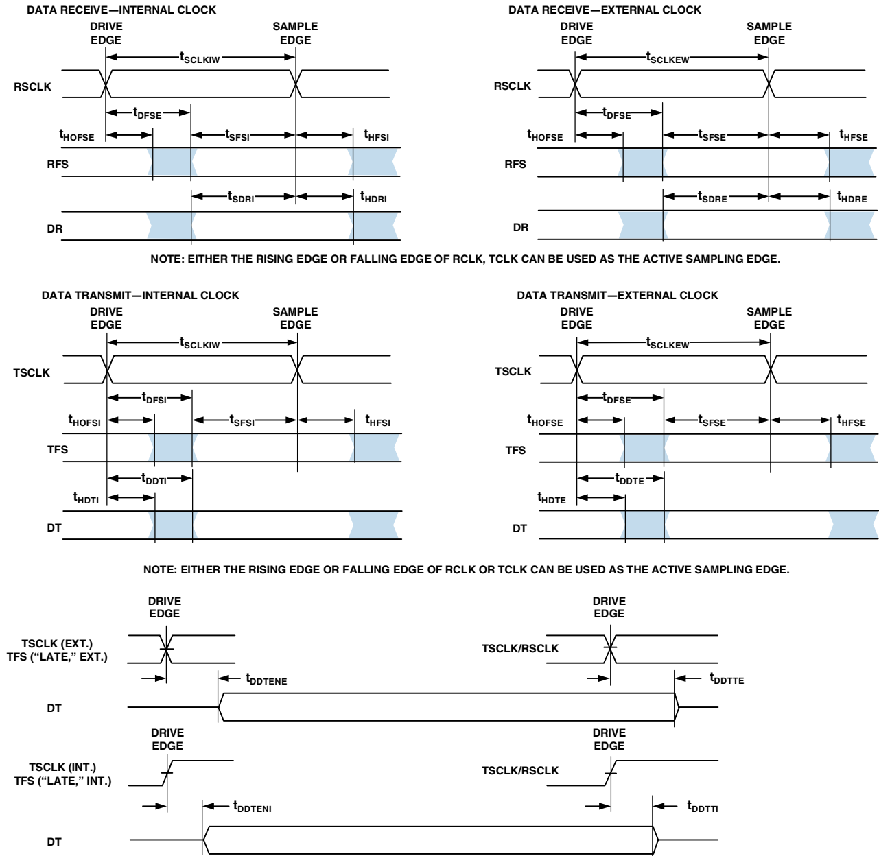
Figure 19. Serial Ports
