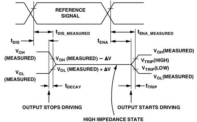
Figure 47. Output Enable/Disable
