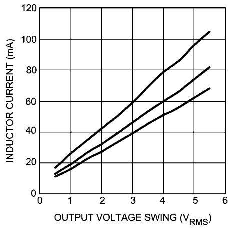
Inductor Current vs Output Voltage Swing 查询"LM48555"供应商 f_s = 10\text{ kHz} , V_{DD} = 3\text{ V}, 4.2\text{ V}, 5\text{ V}
