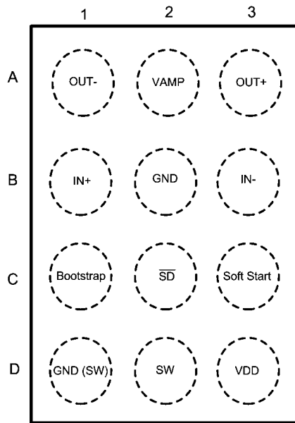
LM48555TL Bumps Down View
