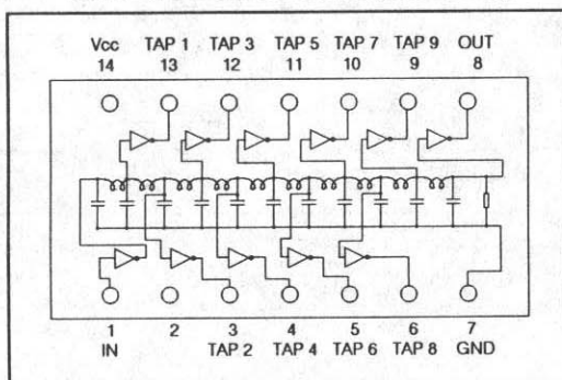
DUAL - IN - LINE PACKAGE (TOP VIEW)
