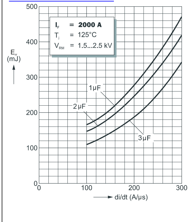
Fig. 11 Turn-off energy vs. turn-off di/dt for I_F = 2000 \text{ A} (max. values).
