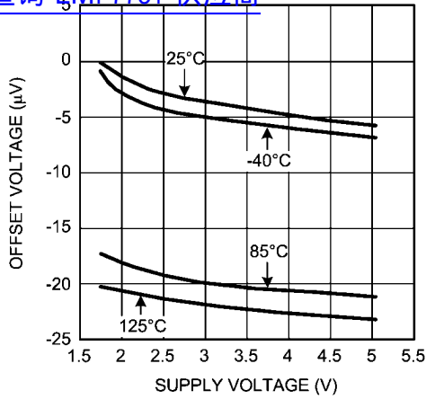
Offset Voltage vs. Supply Voltage 查询"LMP7731"供应商
