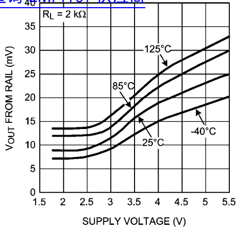
Output Swing Low vs. Supply Voltage 查询"LMP7731"供应商
