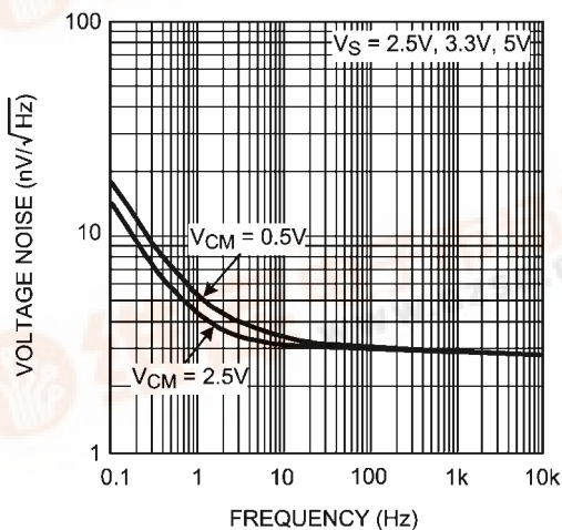
Input Voltage Noise vs. Frequency
