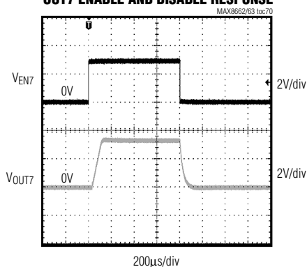
OUT7 ENABLE AND DISABLE RESPONSE
