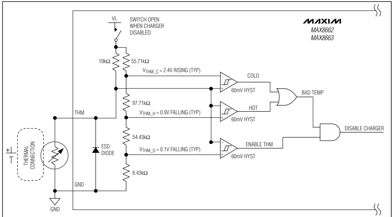
Figure 6. Thermistor Input
