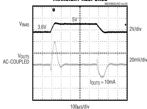
OUT5 REGULATOR LINE-TRANSIENT RESPONSE
