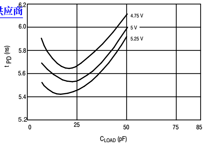
Figure 9. t_{PD} versus Load Typical at T_A = 25^\circ\text{C}
